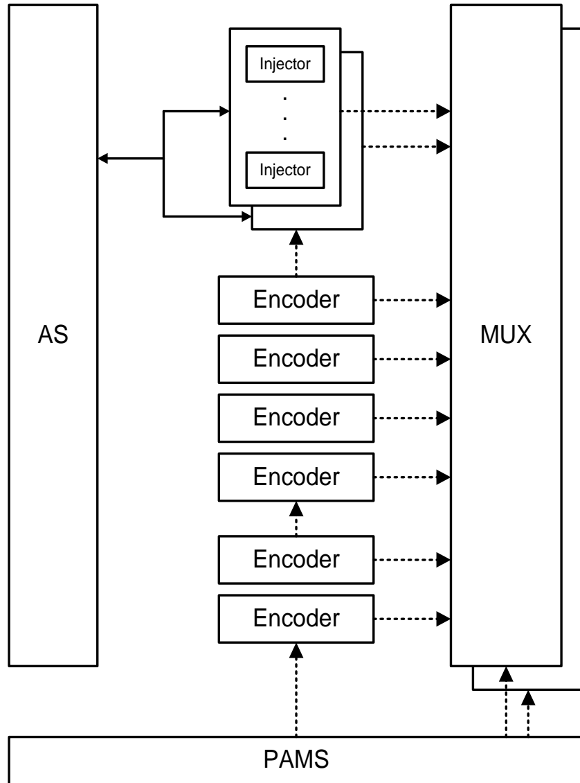
Figure 12-6 - Two-way Block Diagram with External Injector
