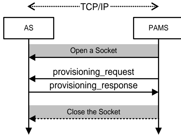
Figure 12-18 - PAMS detects an Injector Failure
