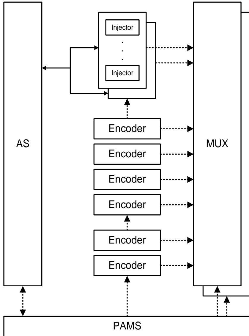
Figure 12-15 - Two-way Block Diagram with External Injector
