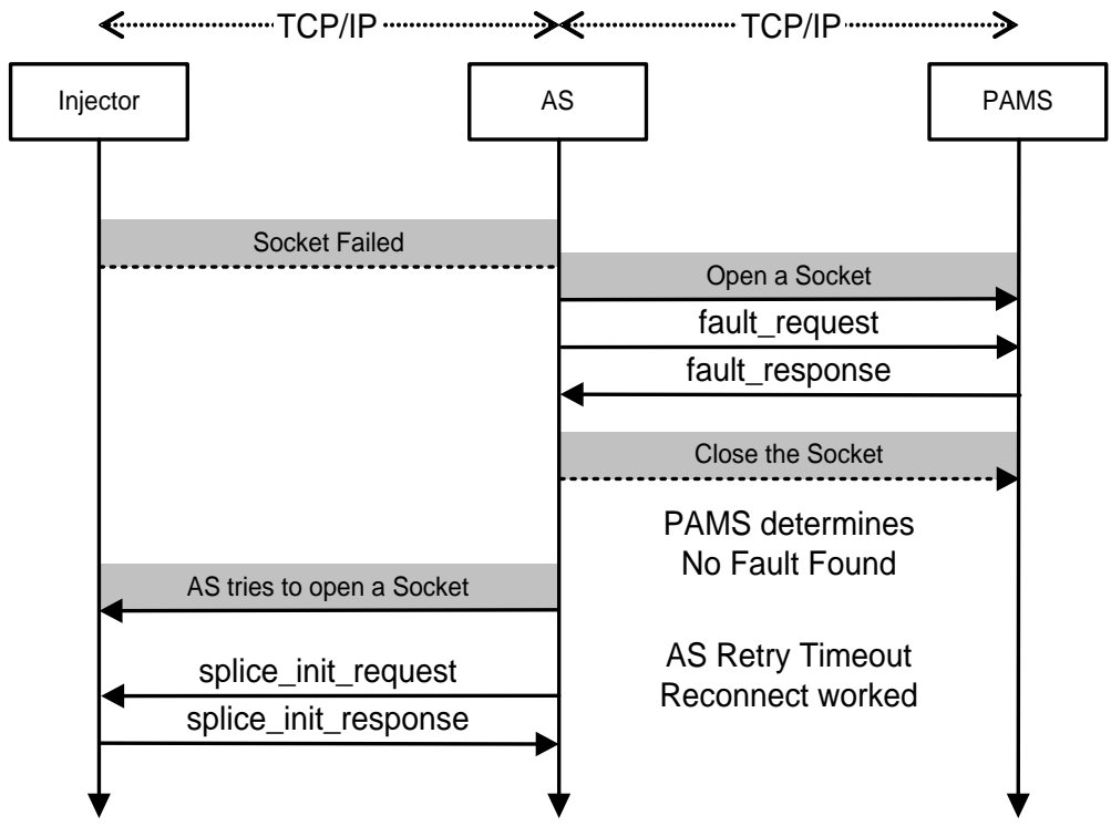
Figure 12-20 - Injector Socket Failed and Recovered
